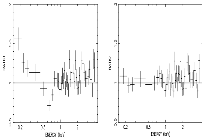
Fig. 2. An absorption feature and a soft excess are clearly evident in the LECS residuals when a power law ( \Gamma = 1.57 , N_H = N_H^{Gal} ) is fitted the the data ( left panel ). Data are well parameterized by a broken power-law plus a notch ( right panel )
