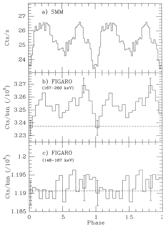
FIG. 3.—Light curve of A0535+26 in the energy range (32–91) keV as observed by SMM (Sembay et al. 1990) (a) and those obtained from the FIGARO data at 103.2 s in the energy ranges (167–260) keV (b) and (148–167) keV (c). The dashed lines indicate the background levels as derived from the template light curve and used to compute the pulsed flux.
