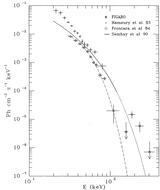
FIG. 4.—Spectrum of the pulsed emission of A0535+26 in the low-energy gamma rays as measured by FIGARO. Data from previous hard X-ray measurements, both pulsed (Frontera et al. 1984) and total (Hameury et al. 1983) are also shown; the solid line is the spectrum given by Sembay et al. (1990).
