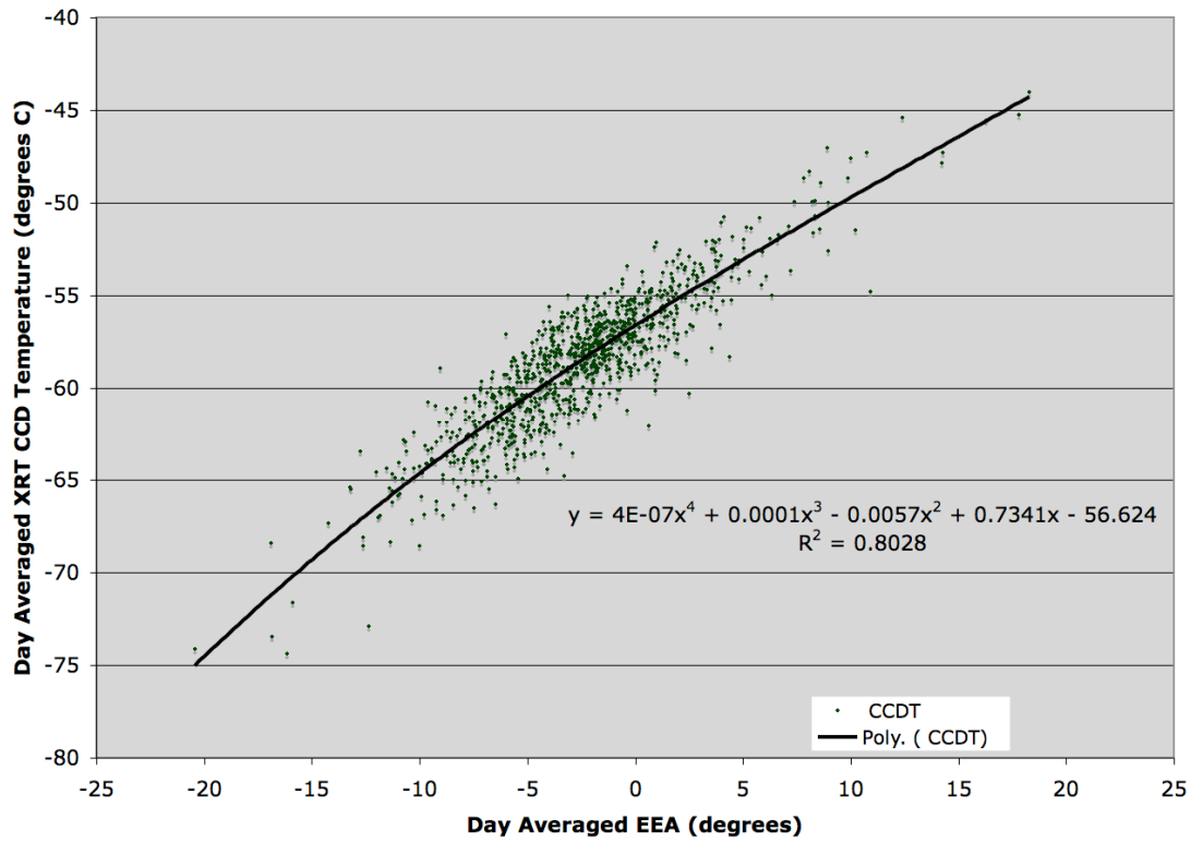
Figure 1. An updated model for estimating the XRT CCD temperature as a function of Earth Elevation Angle.
