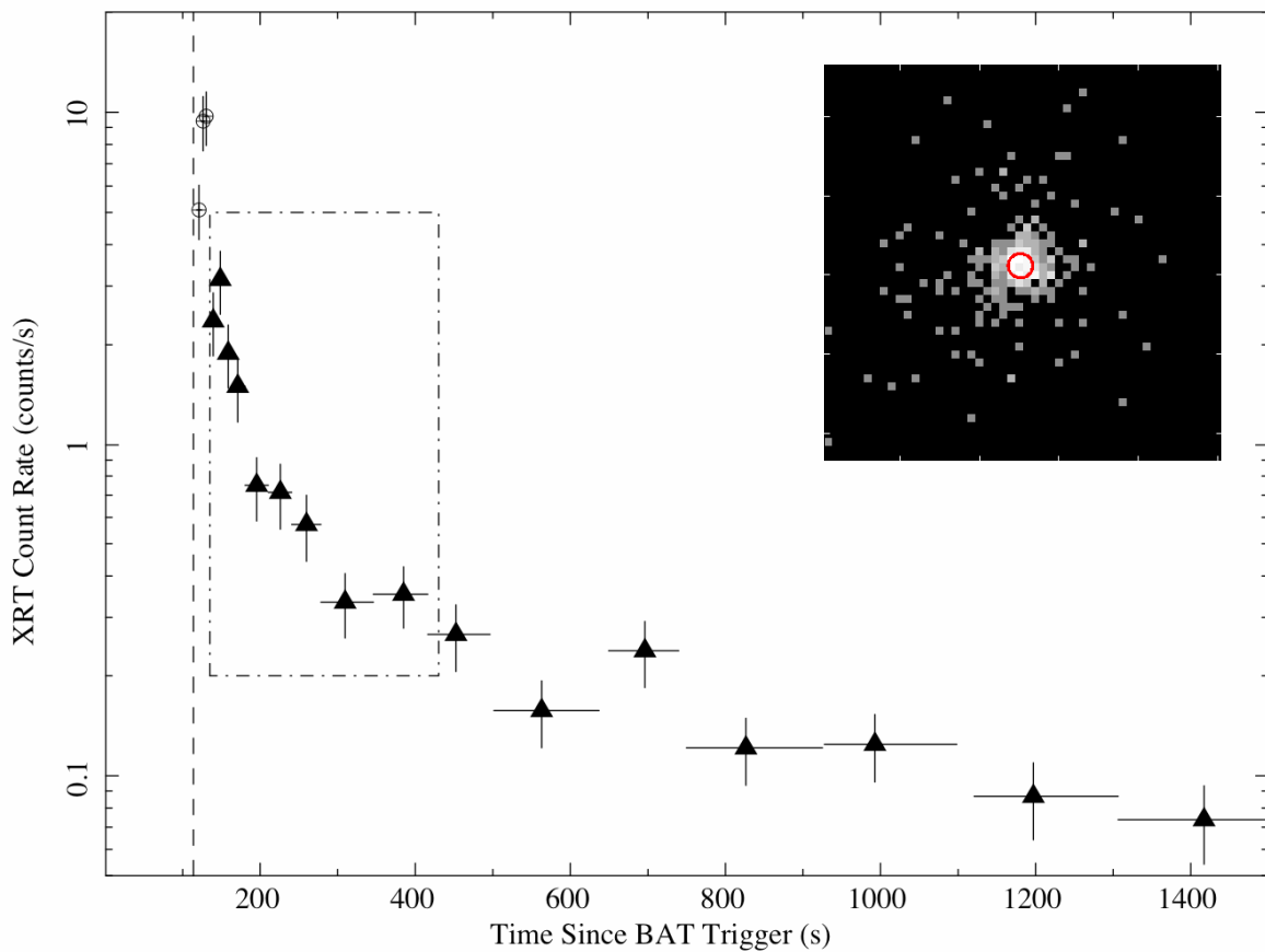
Figure 3. XRT light-curve of the X-ray afterglow of GRB070808. The vertical dashed line represents the time at which the XRT took a 2.5s image of the field and attempted to produce a rapid position through centroid. The points on the light-curve represent the X-ray afterglow brightness in data in WT mode (circles) and PC mode (triangles). The dot-dash box represents the time period in which the first batch of SPER data are being taken. (Inset) Image formed from SPER data on GRB 070808. The error circle plotted on this image is the calculated centroid position and 90% confidence level error circle calculated from the data taking the location of hot columns into account.
