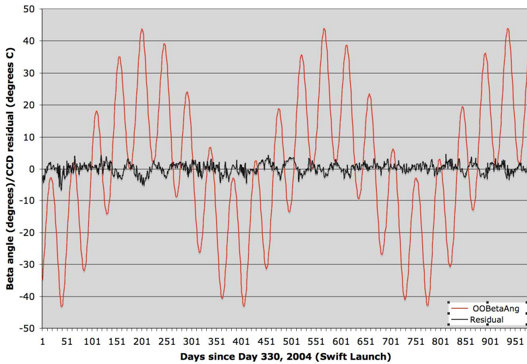
Figure 2. Residuals from the model show in Figure 1 (black) and the \beta -angle (sinusoidal line) for the first 1000 days of XRT operation.
