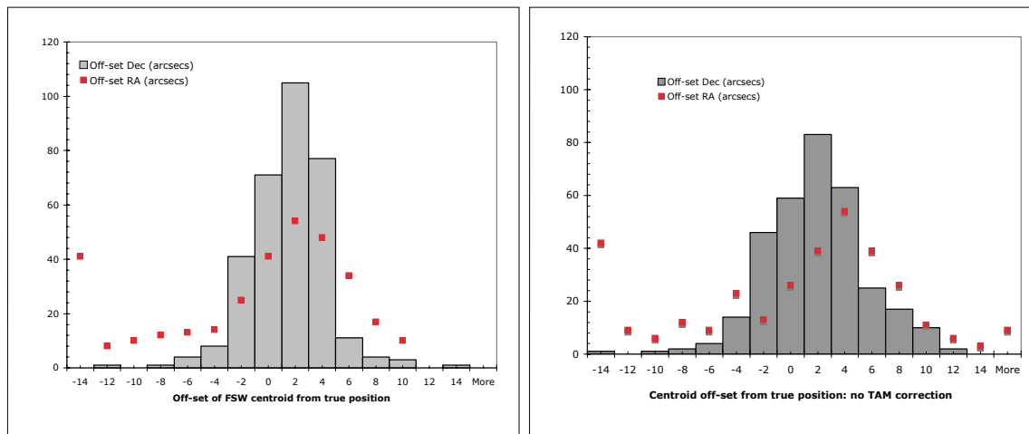
Figure 3.3 Histograms of the difference in RA and DEC between the J2000 positions and the FSW obtained centroids including the TAM correction (left) and the FSW centroids with no TAM correction (right)
