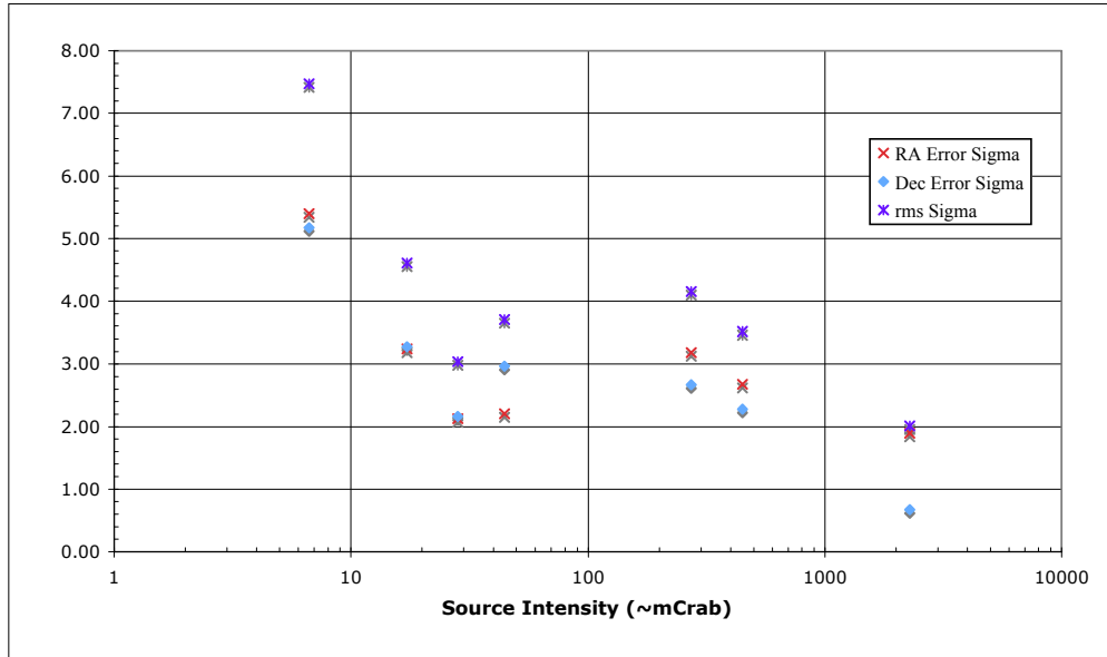
Figure 3.2 XRT centroiding accuracy versus source intensity (uncorrected for pile-up), where the XRT response is \sim 0.7 counts/mCrab 4
