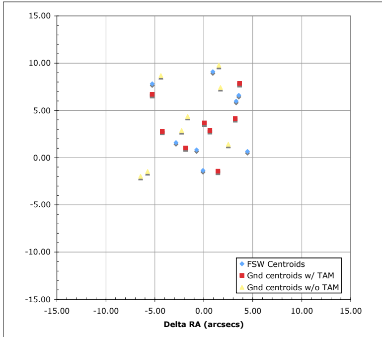
Figure 3.4 Differences in the RA and DEC in arcseconds between the XRT TDRSS position and the ground position of the optical counterpart
